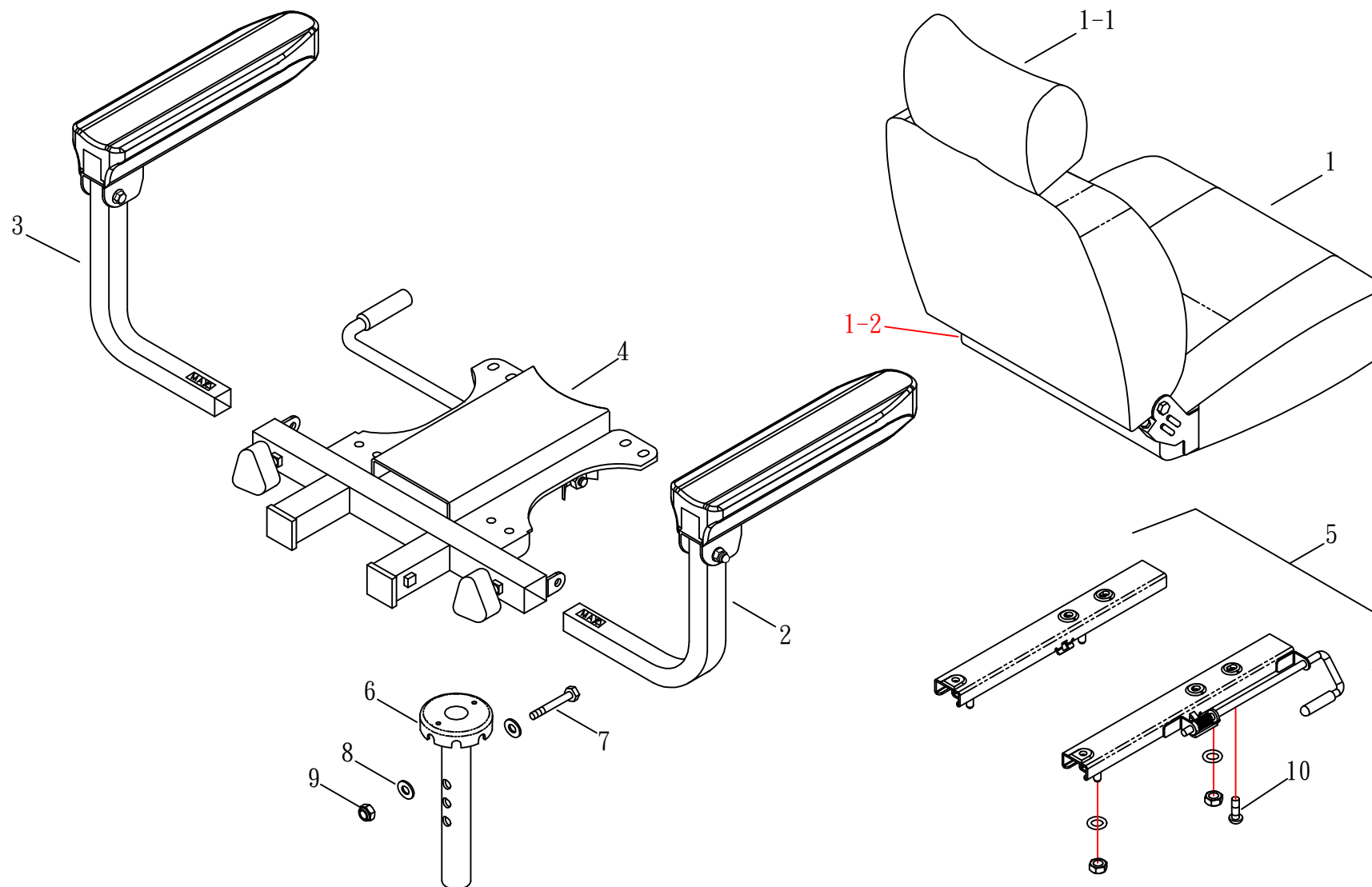
(FIG. 4) SEAT
